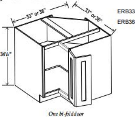
Easy Reach Base Cabinet
