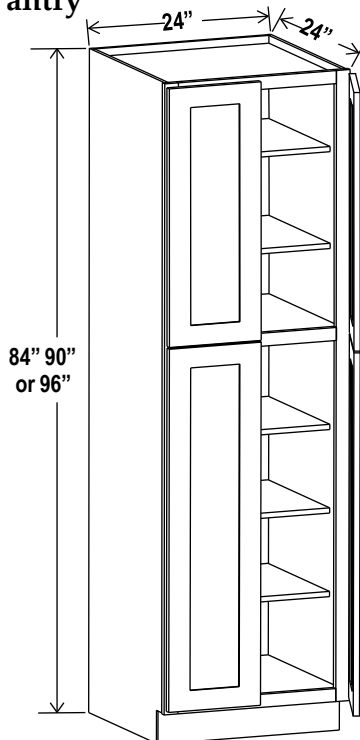
Utility Pantry
