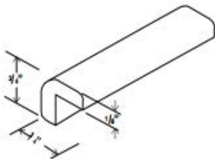
Scribe Moulding
