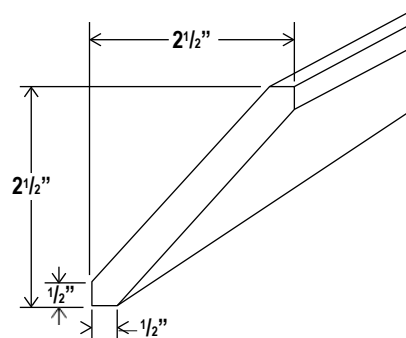
Angle Crown Moulding
