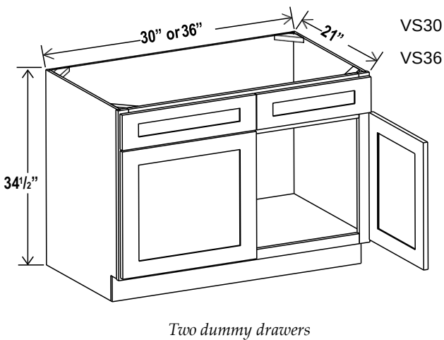
Vanity Sink Base
