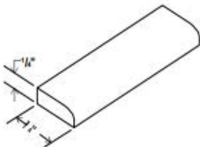
Scribe Moulding
