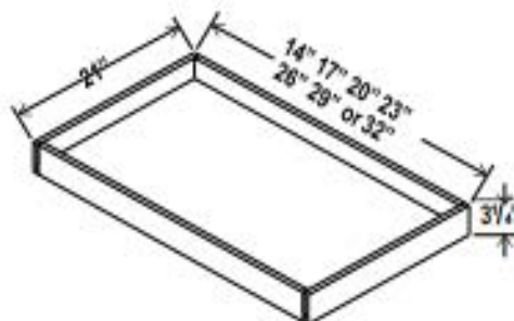
Roll Out Tray
