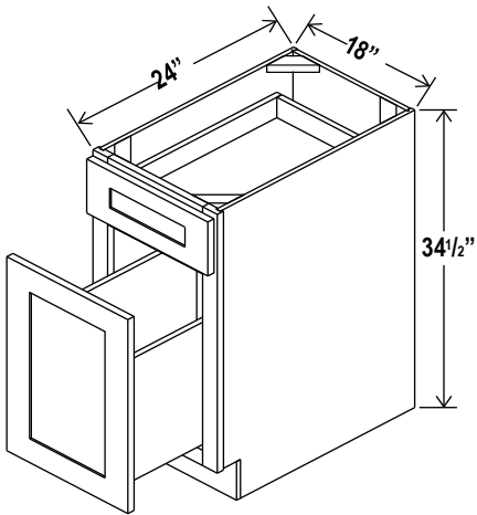
Spice Pull Base Cabinet
