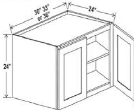
Refrigerator Wall Cabinet Double Doors
