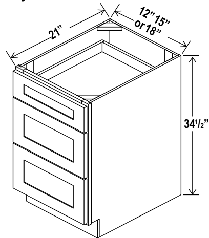
Vanity Drawer Base Cabinet
