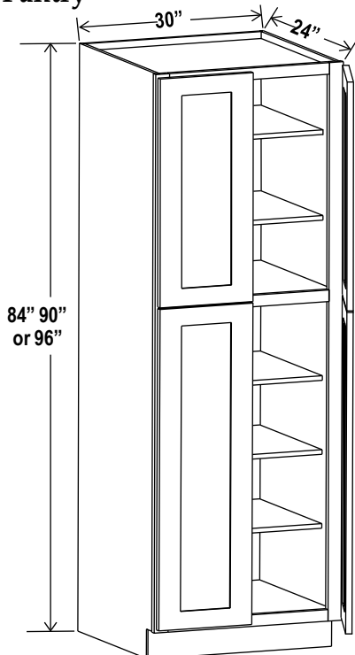
Utility Pantry
