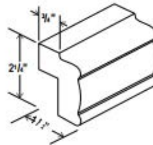
Crown Moulding
