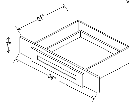
Knee Drawer
