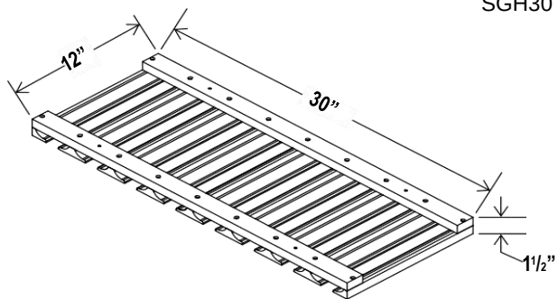
Glass Holder
