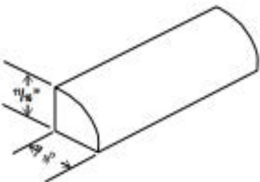
Shoe Moulding
